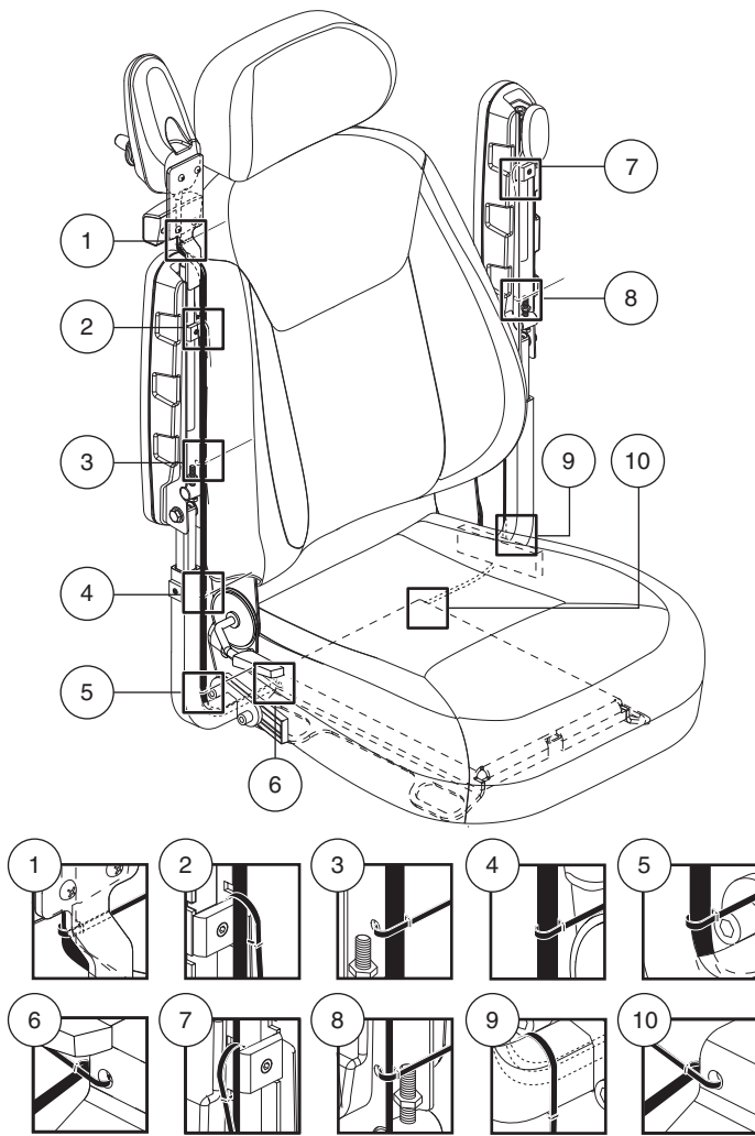
Figure 10. Controller Harness Routing on a Captain's Seat with iLevel
