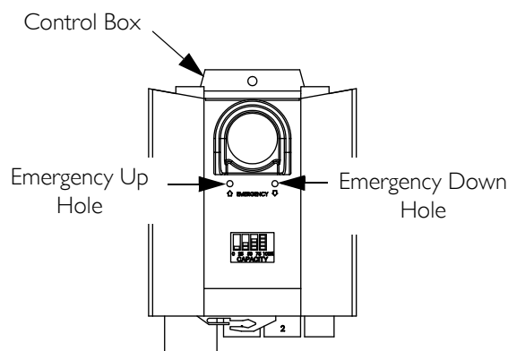
FIGURE 3.2 Primary Emergency Release
